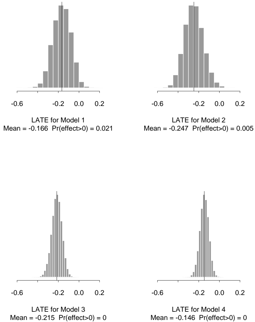
Figure 2: Posterior distribution of the local average treatment effects of catheterization on mortality from our four instrumental variable models. The local average treatment effect is defined as the average mortality when all patients undergo catheterization less the average mortality when all patients do not undergo catheterization for patients who are inferred to potentially receive both treatments. The solid vertical line corresponds to the posterior means.
